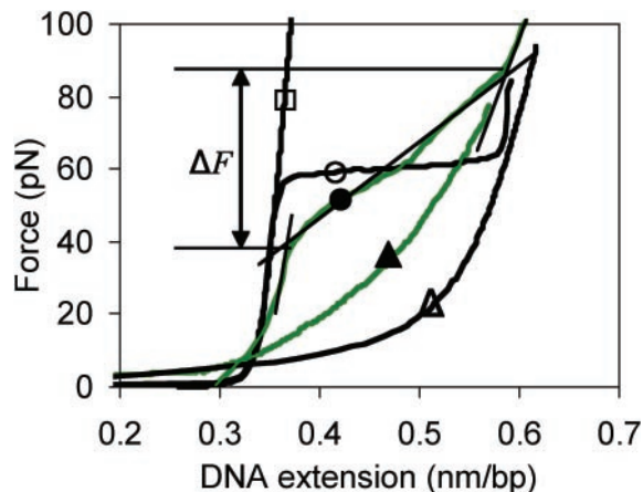
Figure 3. Stretching curves for \lambda -DNA in the absence of protein (open circle), in the presence of 20 nM NCp7 (wild type) protein (closed circle), and for ssDNA with NC bound on it (closed triangle), all in FIM buffer (see Materials and Methods) and room temperature. For ssDNA with NC bound, data are from ref. (35), and was taken with 10 nM NCp7 in 25 mM NaCl, 10 mM HEPES, pH 7.5, room temperature. Stretching curves for dsDNA (open square) and ssDNA (open triangle), fit to standard polymer models, in the absence of protein (90) are also shown. The method used to determine \Delta F , the force transition width, is shown schematically.
