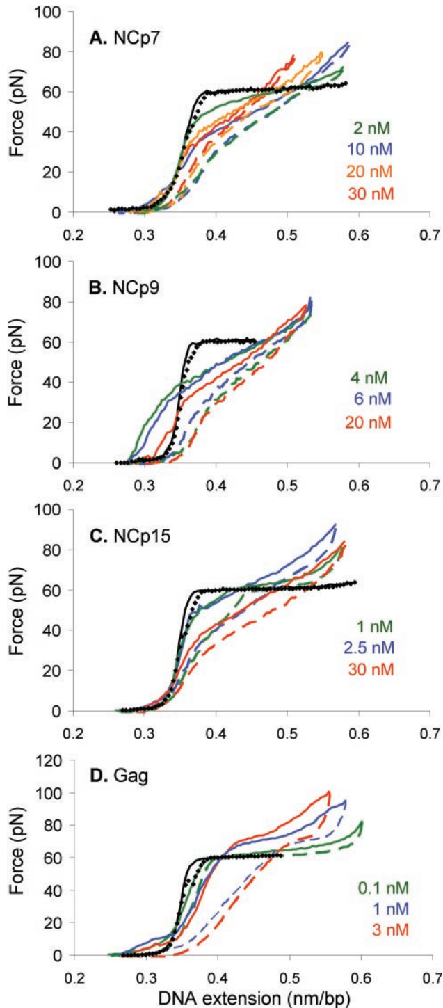
Figure 5. Stretching (solid lines) and relaxing (dashed lines) curves for \lambda -DNA in the presence of the NC proteins or Gag: (A) NCp7; (B) NCp9; (C) NCp15; (D) Gag. Protein concentrations are indicated in the figure. Data were collected in FIM buffer (see Materials and Methods) at room temperature. The stretching and relaxing curves in the absence of protein are also shown (black solid line and filled diamonds, respectively).
