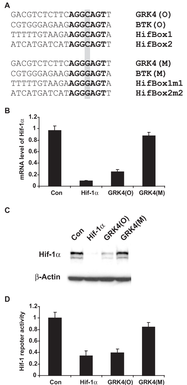
Figure 3. The 7 nt motif in GRK4(O)/BTK(O) is responsible for the off-target silencing of HIF-1 \alpha . (A) Sequence alignment of the original GRK4 and BTK siRNAs, the two 7 nt boxes (HifBox1 and HifBox2) in the hif-1 \alpha mRNA that is complementary to the original GRK4 and BTK siRNAs and the mutated GRK4 siRNA, BTK siRNA, HifBox1 and HifBox2 that carry a C to G change to disrupt the 'AGGCAGT' motif. GRK4(O) and BTK(O) represent the original GRK4 and BTK siRNAs in the kinase siRNA library. GRK4(M) and BTK(M) represent siRNAs with a C to G mutation as compared to GRK4(O) and BTK(O). HifBox1m1 and HifBox2m2 represent mutated sequences of the HifBox1 and HifBox2 (each with a C to G mutation compared to HifBox1 and HifBox2). (B) H1299 cells were transfected with indicated siRNAs and collected 24 h later for QPCR analysis of HIF-1 \alpha expression. (C) H1299 cells were transfected with indicated siRNAs for 24 h, treated with 100 \mu M DFO for 6 h and analyzed for HIF-1 \alpha expression using western blotting. (D) H1299 cells were transfected with the dual reporters, pHRE and pRL-TK, transfected with indicated siRNAs 24 h after reporter transfection and subjected to hypoxia treatment for an additional 18 h. Cells were then collected and analyzed using the Dual-Glo luciferase assay system. In all experiments, the siRNAs were transfected using a final concentration of 20 nM.
