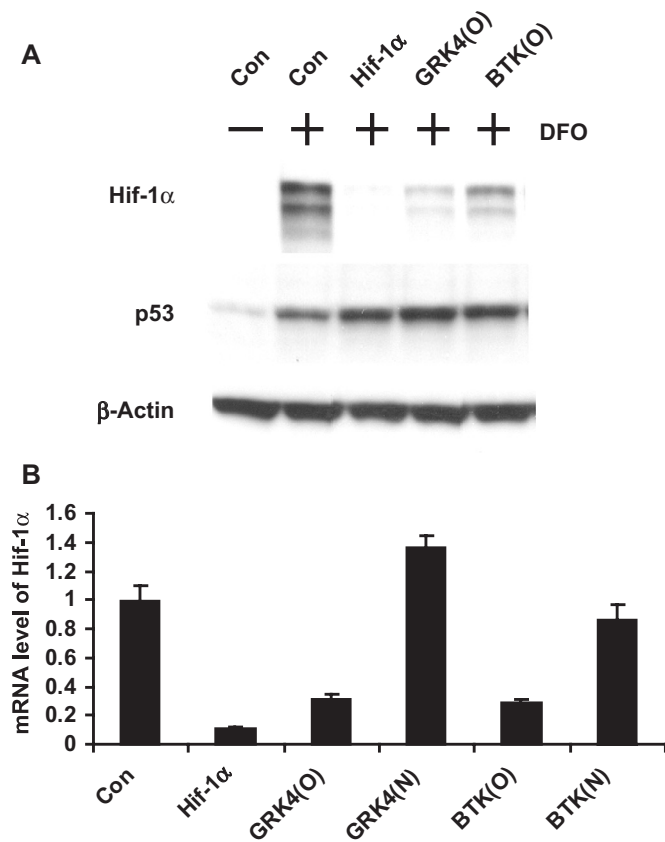
Figure 2. The original GRK4 and BTK siRNAs down-regulates HIF-1 \alpha at both protein and mRNA levels. (A) H1299 cells were transfected with indicated siRNAs for 24 h and subjected to 100 \mu M DFO treatment (+) or mock treatment (-) for an additional 6 h. The cells were collected and analyzed by western blotting using antibodies against HIF-1 \alpha , p53 and \beta -actin. (B) H1299 cells were transfected with indicated siRNAs, collected 24 h after transfection and analyzed by QPCR for HIF-1 \alpha expression. In all experiments, the siRNA were transfected using a final concentration of 20 nM. The original GRK4 and BTK siRNAs were designated as GRK4(O) and BTK(O). The new GRK4 and BTK siRNAs were designated as GRK4(N) and BTK(N). Con and HIF-1 \alpha represent the control siRNA and the HIF-1 \alpha siRNA, respectively.
