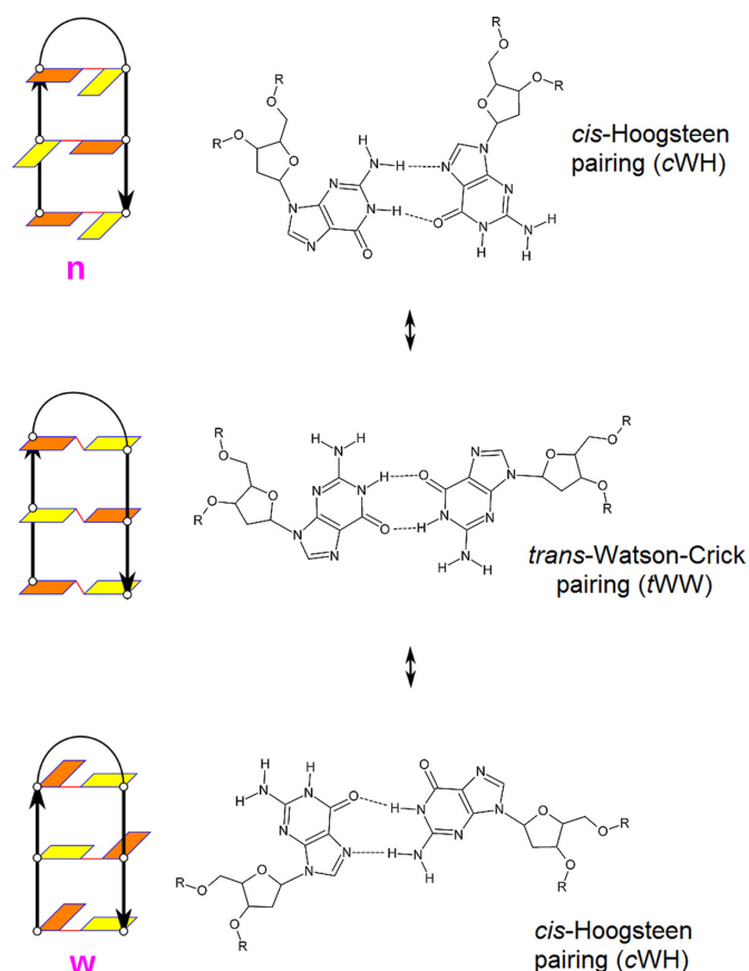
Figure 2. Three types of antiparallel hairpins: narrow groove lateral loop hairpin with c WH pairs (top), diagonal hairpin with t WW pairs (middle) and wide groove lateral loop hairpin with c WH pairs (bottom). The structural schemes are visualized as in the Figure 1.
